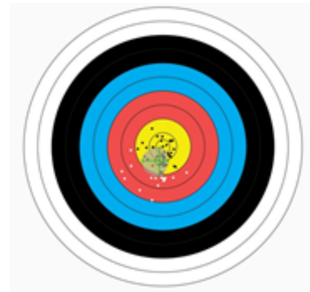
Arrow Dispersion
